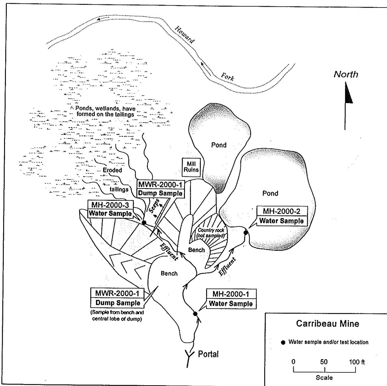
Figure 50. Sketch map of the surface at the 13 th level of the Carribeau Mine.
