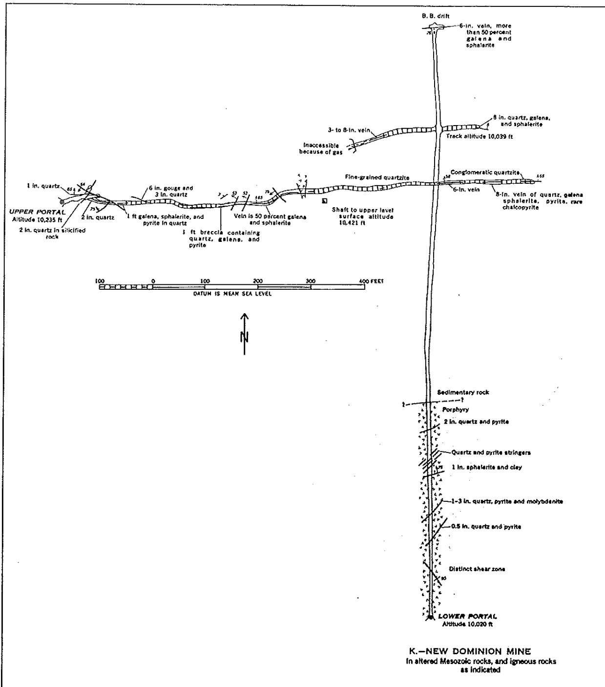
Figure 27. Map of underground workings in the New Dominion Mine, 1942. (Modified from Vhay, 1962, plate 21.)
